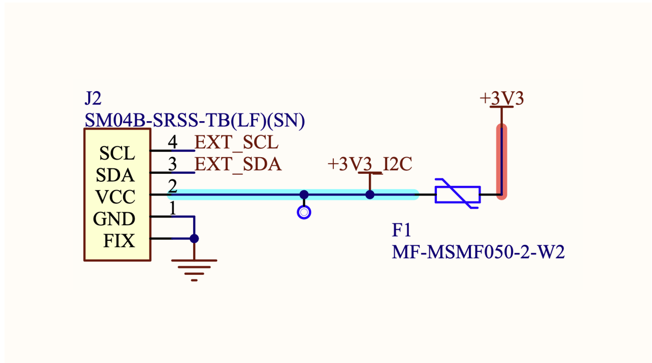
I2C connector.
